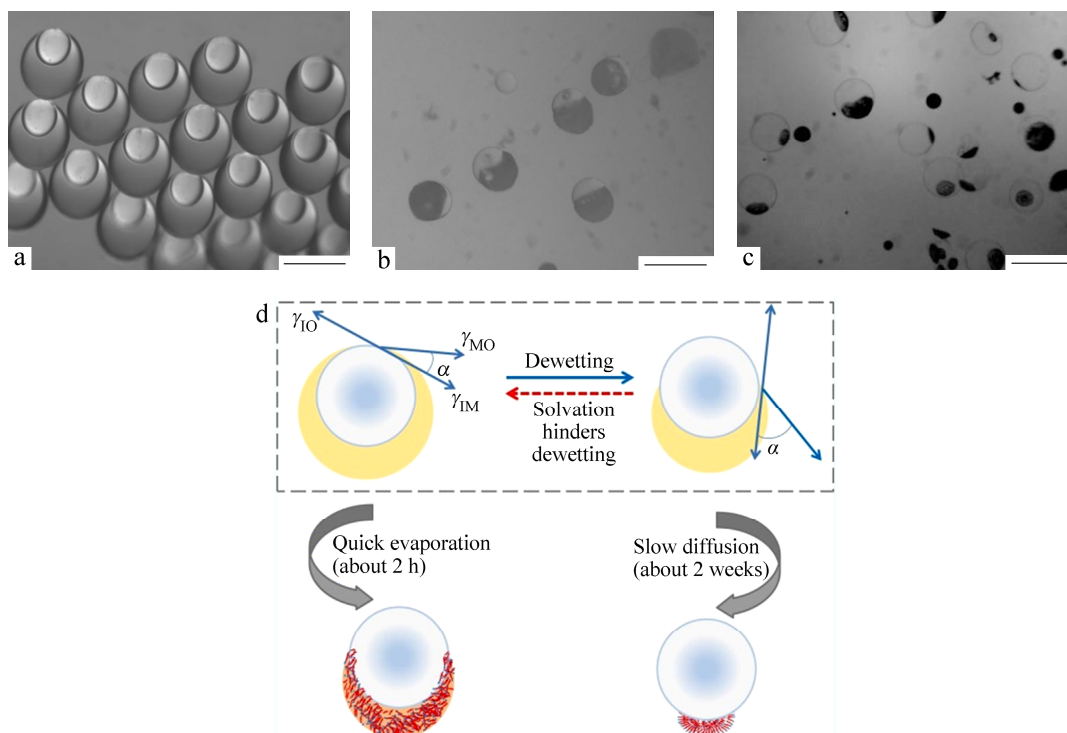
Fig. 3 (a) Off-center droplets (side view), (b) acorn-like vesicles collecting in 10 wt% PVA, (c) patched vesicles collecting in water, (d) illustration of droplets to polymersomes transformation with solvent evaporation and diffusion (Scale bars are 500 \mu\text{m} .)
